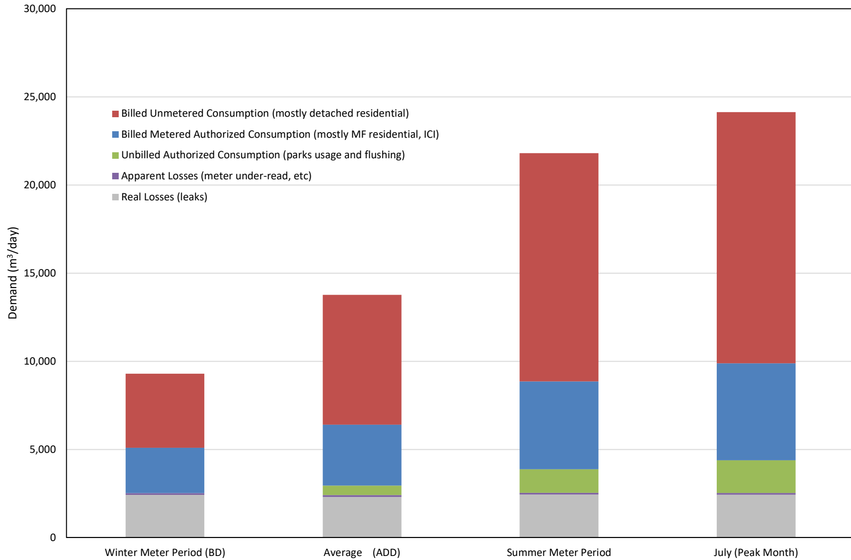
Figure 2-2: City of Courtenay Water Balance (2017)
